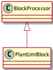
Figure 1.3. The PlantUML block extension class
